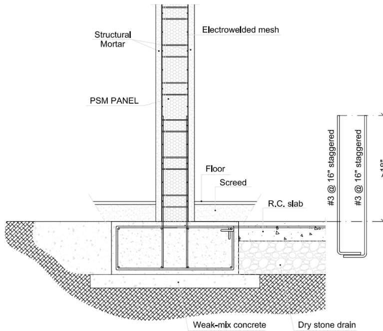
Detail B2. Anchoring to a Beam Foundation
